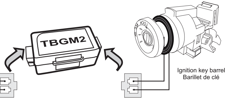
ANTENNA-RING ANTENNE-ANNEAU
